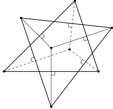
4.9.18) Steiner's theorem
