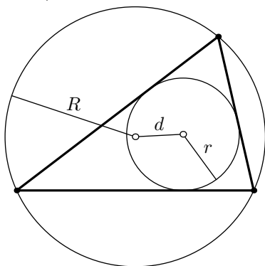
4.6.3) Euler's formula
