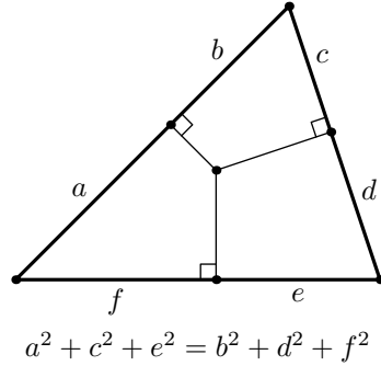
4.9.16) Carnot's theorem
